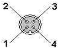
Bayonet Plug, 4 poles, Small (PTB605, CP705, HL2-31/35, HL620)
