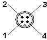
Bayonet Plug, 4 poles, Big (HL920)
